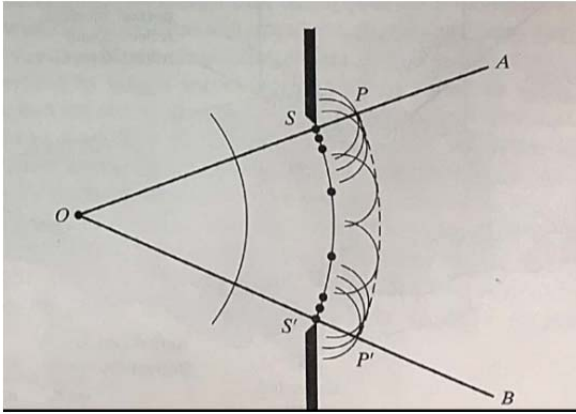
Fig.. 2-3 Huygens' construction for an obstructed wavefront.
